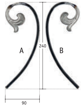
Zierornament
